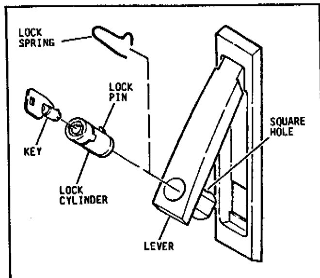
Figure 1-4. Lock Cylinder Installation
